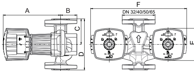
Fig. 5: Flanged pump set
